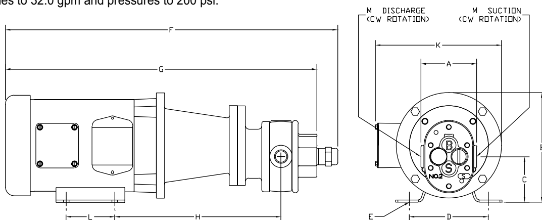
DIMENSIONS (INCHES)
